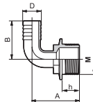
Raccordo portagomma curvo filetto maschio 90° hose fitting with male thread Racor portamangueras curvo rosca macho
