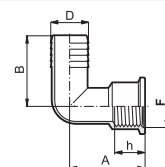
Raccordo portagomma curvo filetto femmina 90° hose fitting with female thread Racor portamangueras curvo rosca hembra
