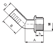
Raccordo portagomma curvo 45° filetto maschio 45° hose fitting with male thread Racor portamangueras curvo 45° rosca macho
